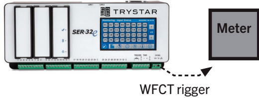
SER, with Trigger Output for Waveform Capture
