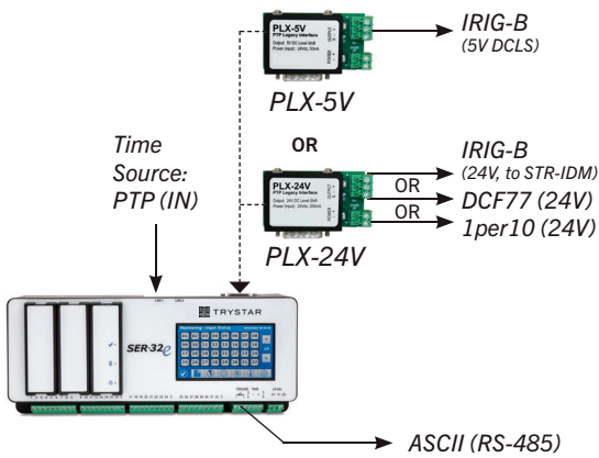
Trystar SER as PTP Slave, with PTP Legacy Interface and ASCII (RS-485) Time-sync Outputs SER-32e
