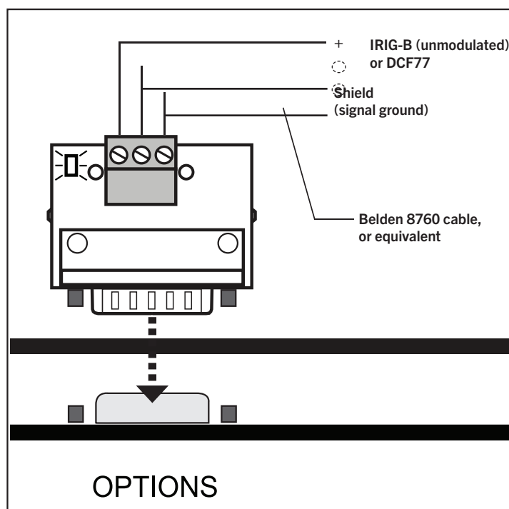
EZC wiring connections (IRIG-B or DCF77) input to Trystar SER
