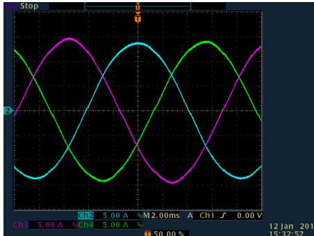
Figure 3 - 100% Load Power
