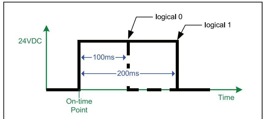
DCF77 pulse-width coding
