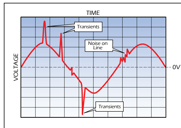
Electrical noise and voltage transients illustrated.
