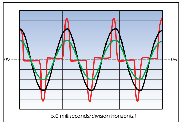
Voltage and Current Waveforms:
